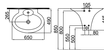
2901-2505 Rena Monoblok Lavabo / Rena Monoblock Washbasin (49x65)
