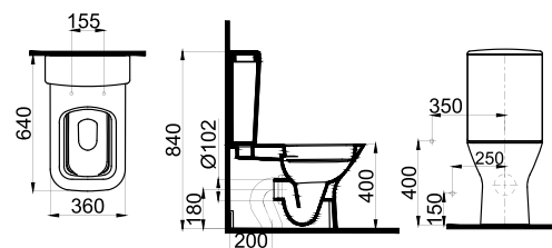
3504-0315 Duvara Sifir Klozet / Back to Wall WC Pan (36x64x40)
