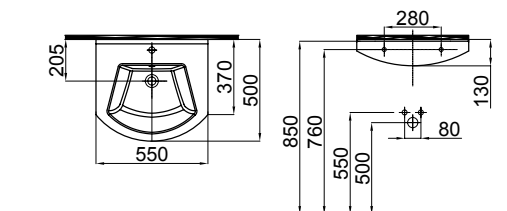
2801-0555 Vega Lavabo / Vega Washbasin (50x55)
