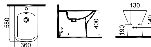
3506-0105 Duvara Sifir Bide / Back to Wall Bidet (36x58x40)
